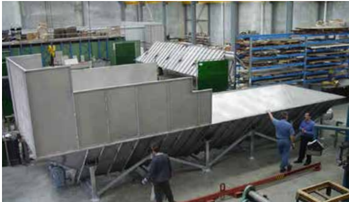
Bins in fabrication in the Perth factory. Hungry boards fitted (but dismantled for shipping)
